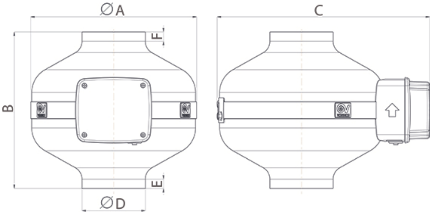
Dimensions (mm)
